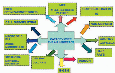
Frequency Planning
